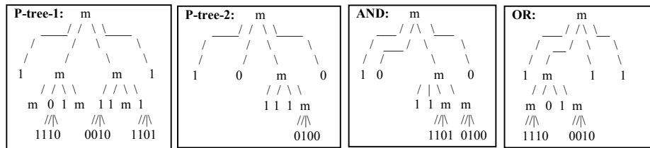
Fig. 2. P-tree Algebra
